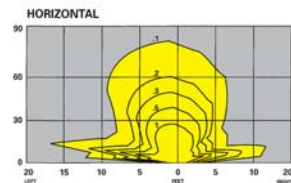
16 12 Volt, 12.0 Watt Halogen Wedge Base
