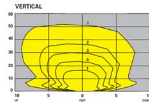
13 6 Volt, 7.0 Watt Halogen Wedge Base
