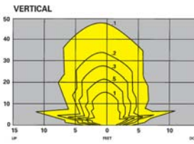
14 6 Volt, 10.0 Watt Halogen Wedge Base
